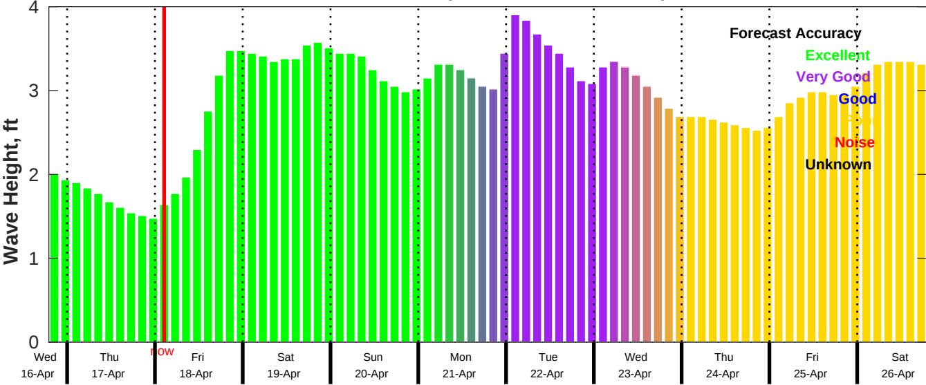
CMEMS Wave Forecast for NDBC 41004 from 16-Apr-2025 19:00:00 to 26-Apr-2025 19:00:00
