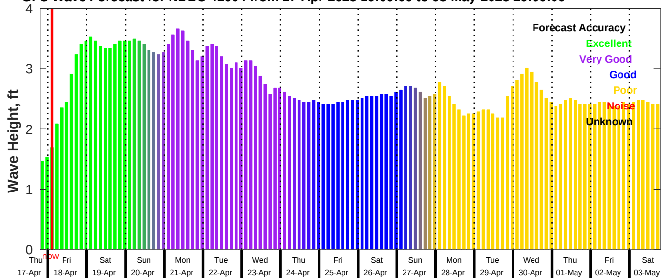
GFS Wave Forecast for NDBC 41004 from 17-Apr-2025 19:00:00 to 03-May-2025 19:00:00
