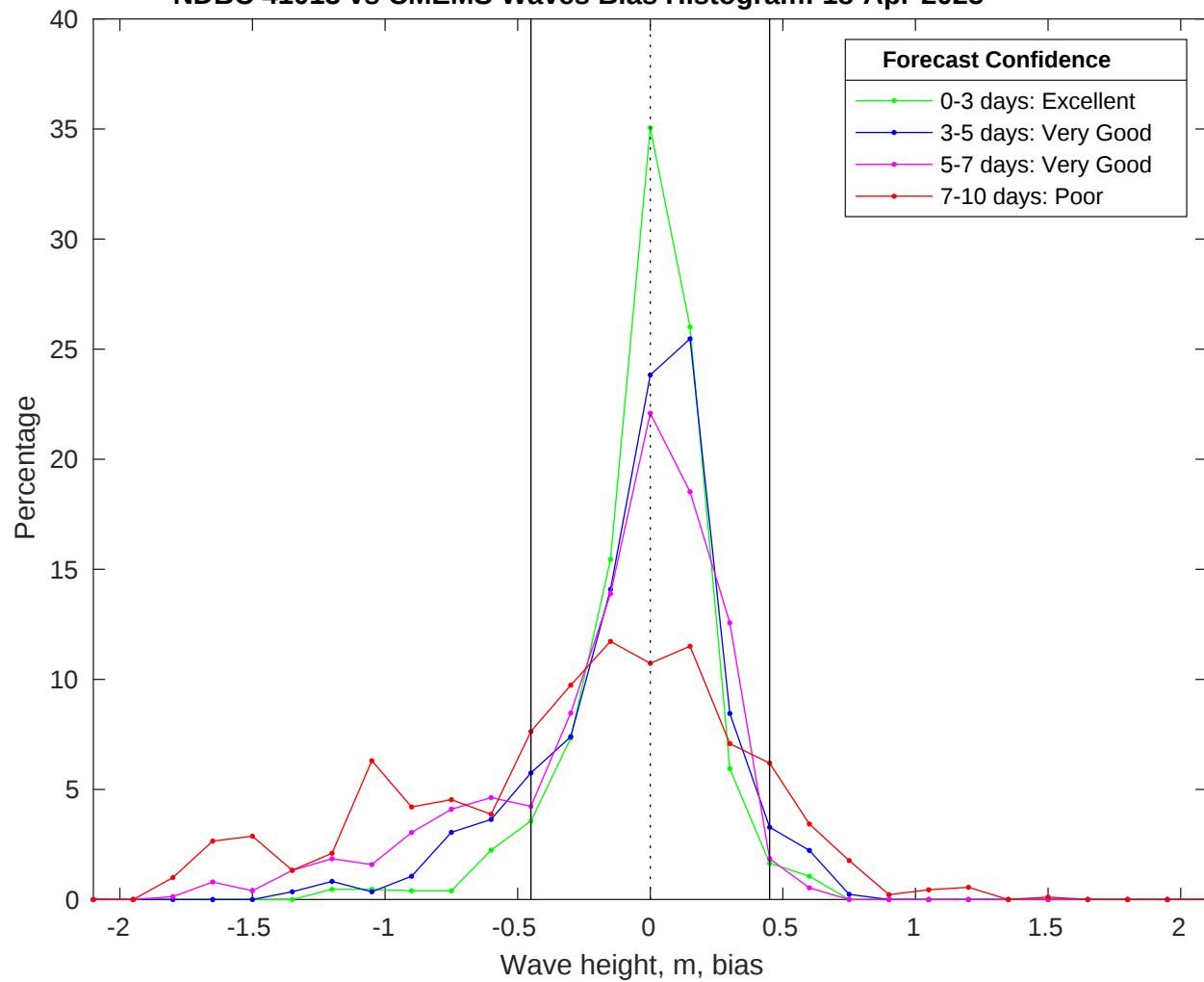
NDBC 41013 vs CMEMS Waves Bias Histogram: 18-Apr-2025
