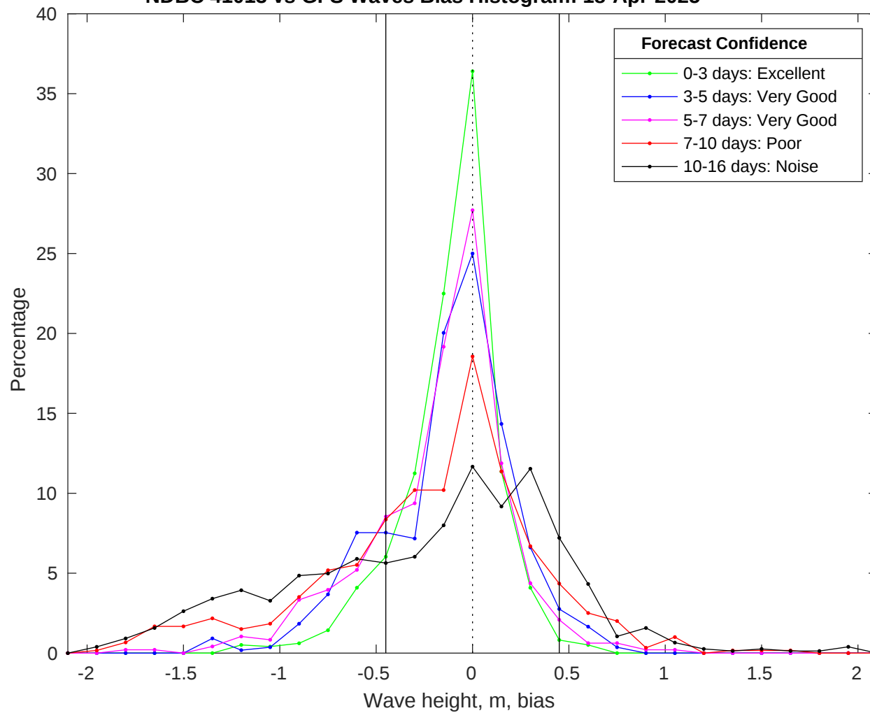
NDBC 41013 vs GFS Waves Bias Histogram: 18-Apr-2025
