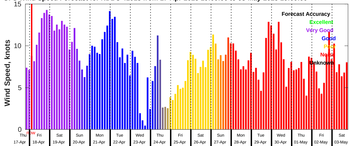
GFS Wind Speed Forecast for NDBC 41013 from 17-Apr-2025 19:00:00 to 03-May-2025 19:00:00
