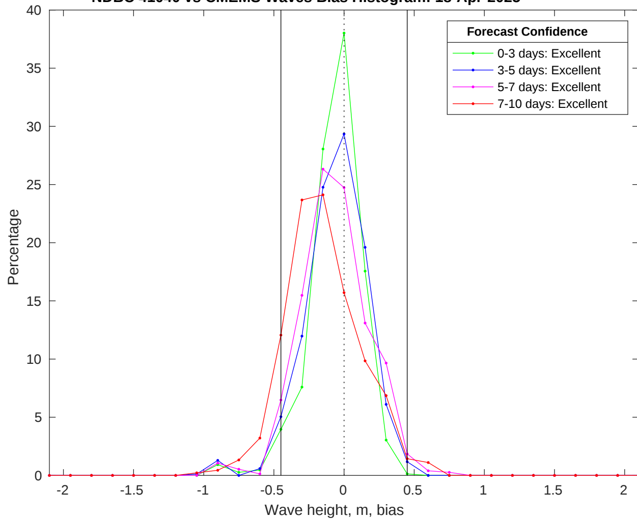
NDBC 41040 vs CMEMS Waves Bias Histogram: 18-Apr-2025
