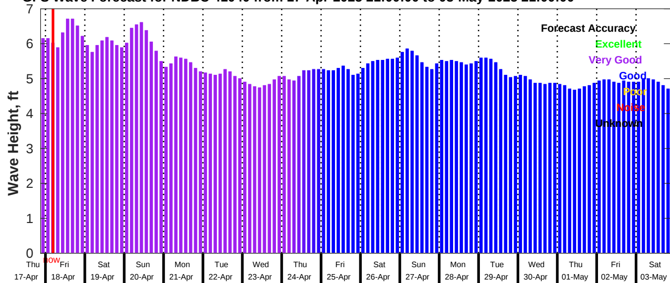
GFS Wave Forecast for NDBC 41040 from 17-Apr-2025 21:00:00 to 03-May-2025 21:00:00
