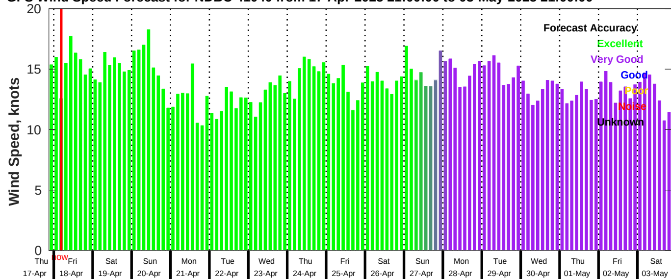
GFS Wind Speed Forecast for NDBC 41040 from 17-Apr-2025 21:00:00 to 03-May-2025 21:00:00
