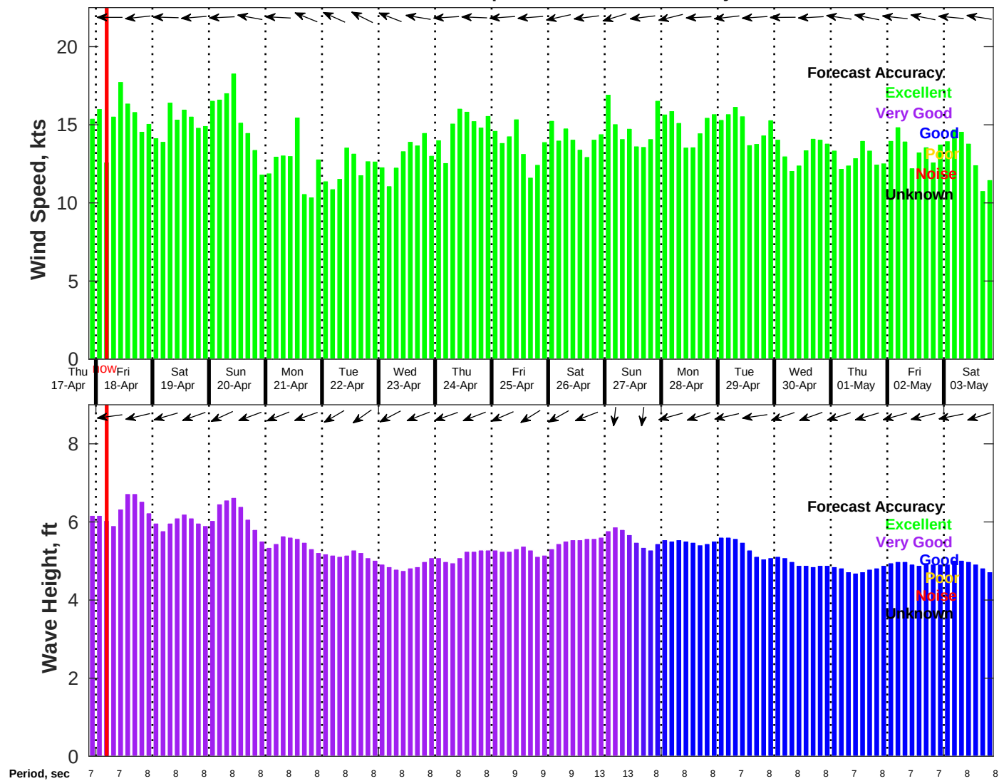
Wind & Wave Forecast for NDBC 41040 from 17-Apr-2025 21:00:00 to 03-May-2025 21:00:00
