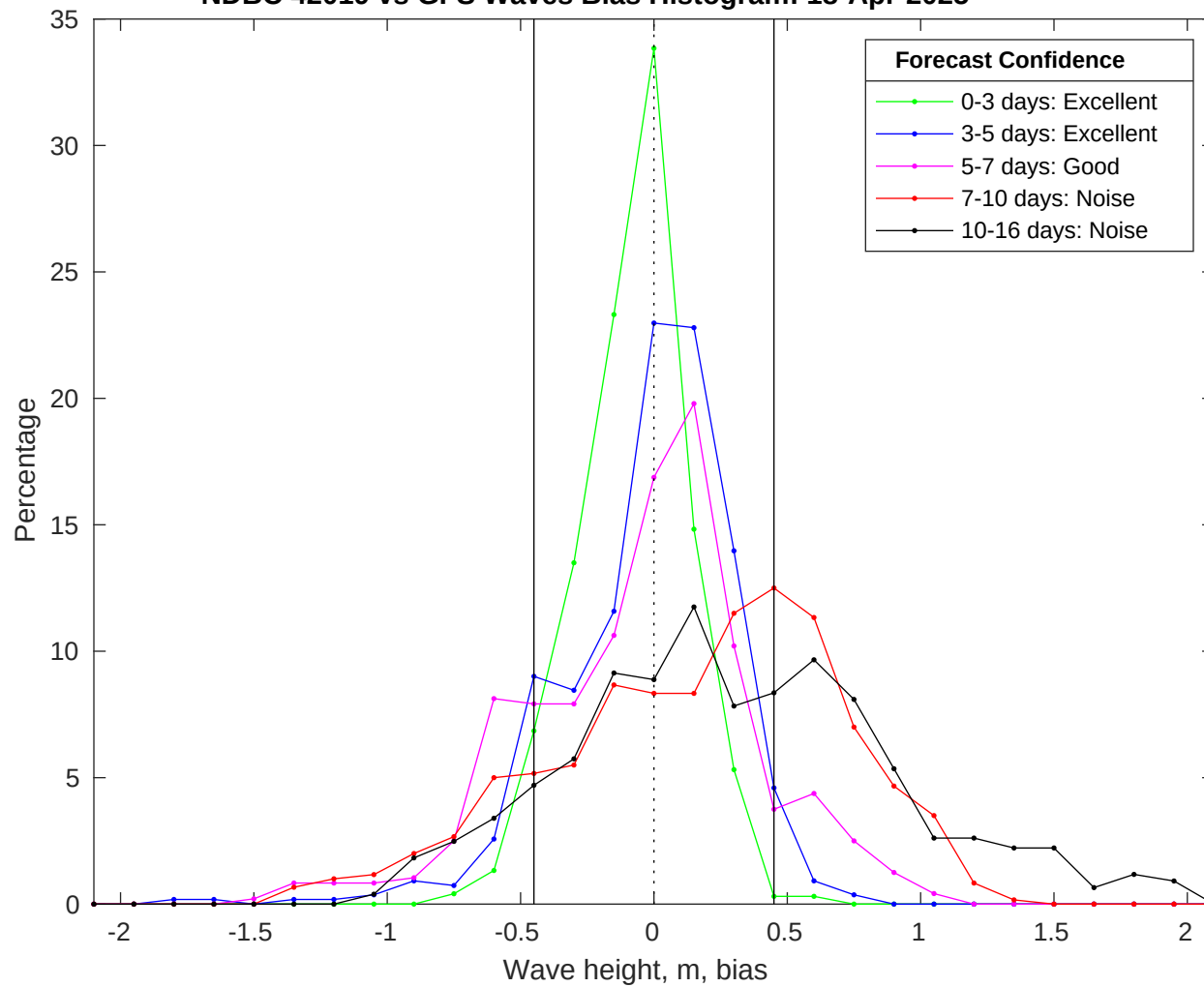
NDBC 42019 vs GFS Waves Bias Histogram: 18-Apr-2025
