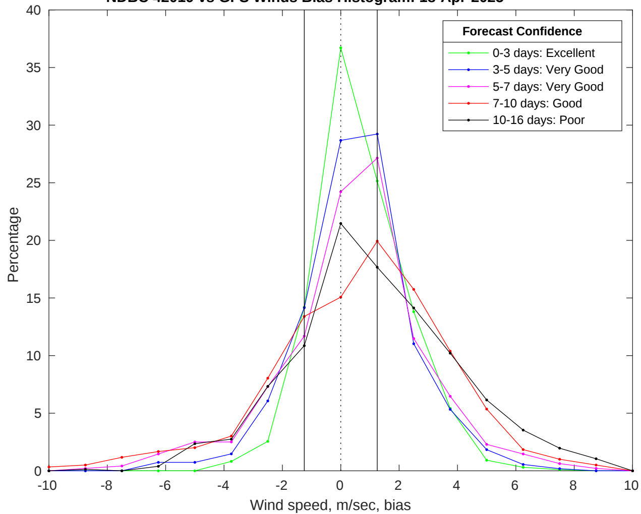
NDBC 42019 vs GFS Winds Bias Histogram: 18-Apr-2025
