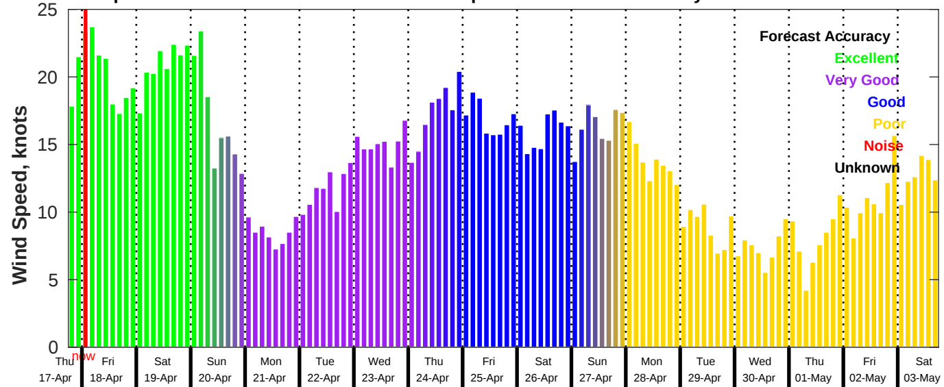
GFS Wind Speed Forecast for NDBC 42019 from 17-Apr-2025 18:00:00 to 03-May-2025 18:00:00
