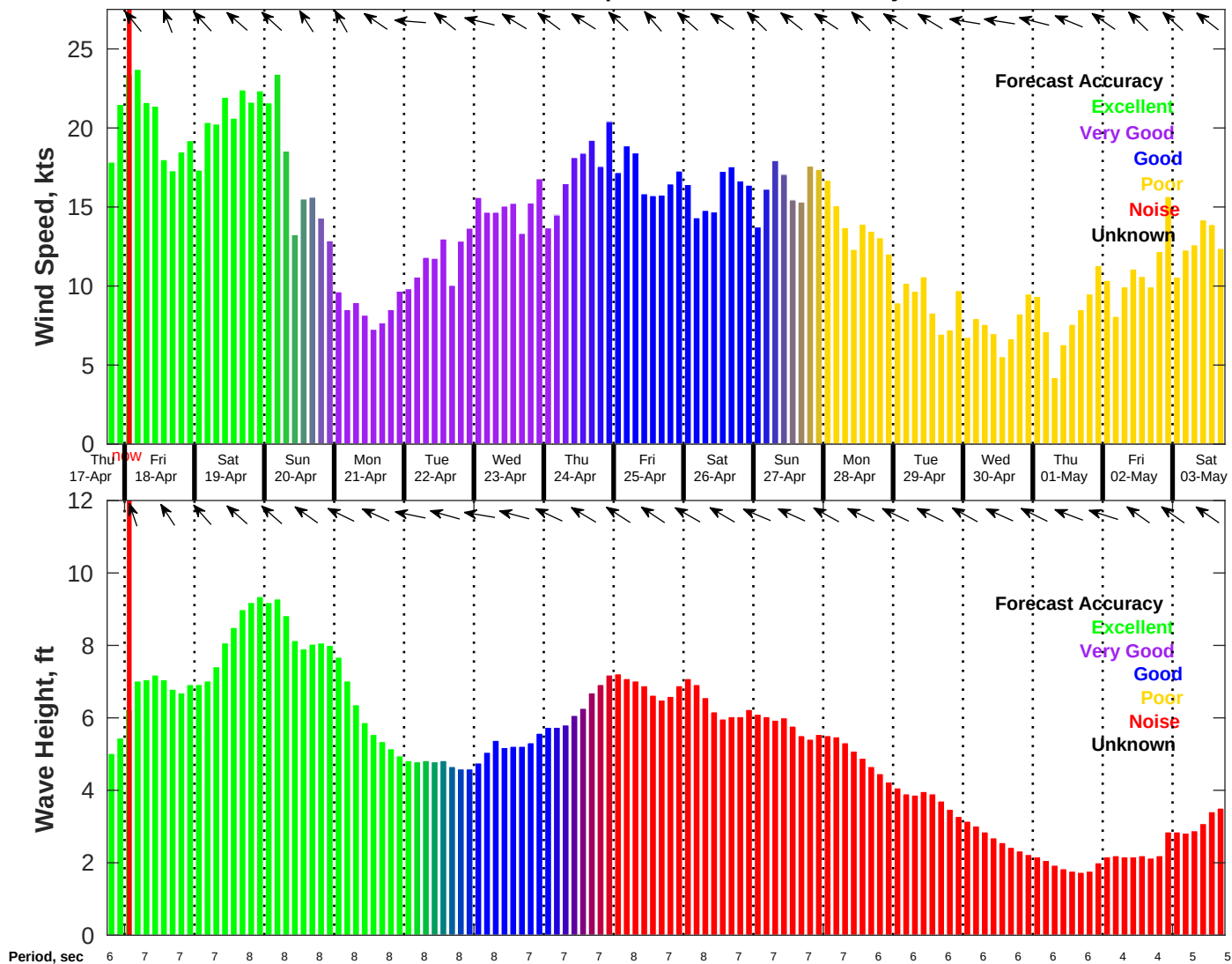
Wind & Wave Forecast for NDBC 42019 from 17-Apr-2025 18:00:00 to 03-May-2025 18:00:00
