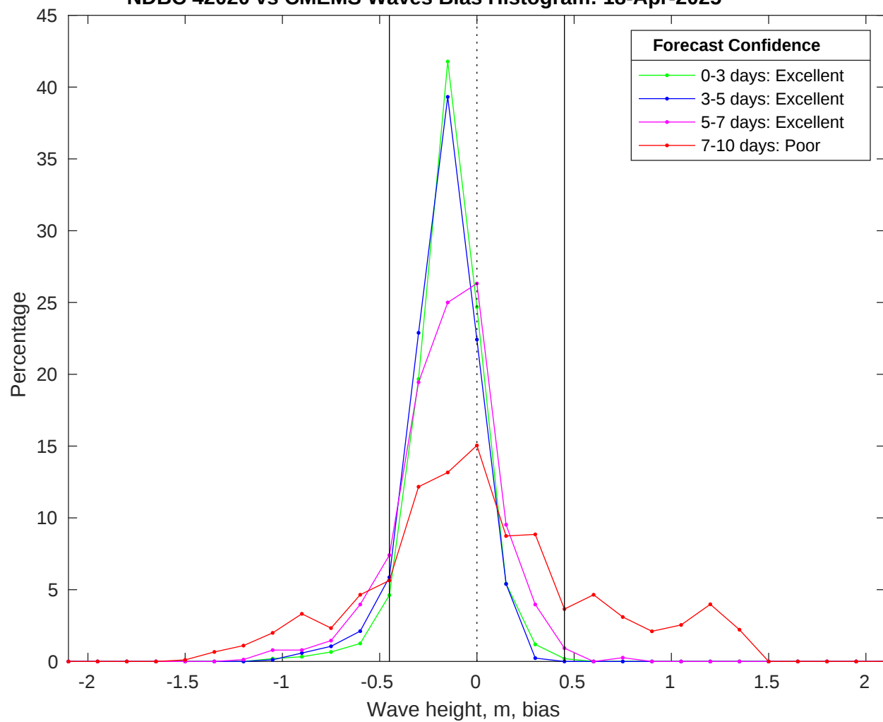
NDBC 42020 vs CMEMS Waves Bias Histogram: 18-Apr-2025
