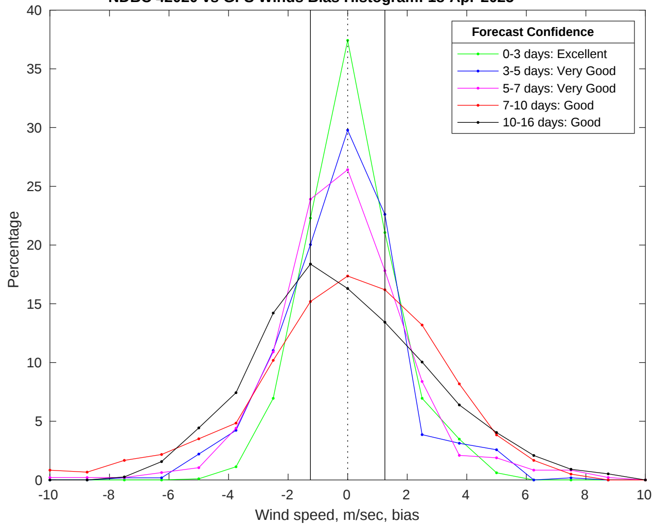
NDBC 42020 vs GFS Winds Bias Histogram: 18-Apr-2025
