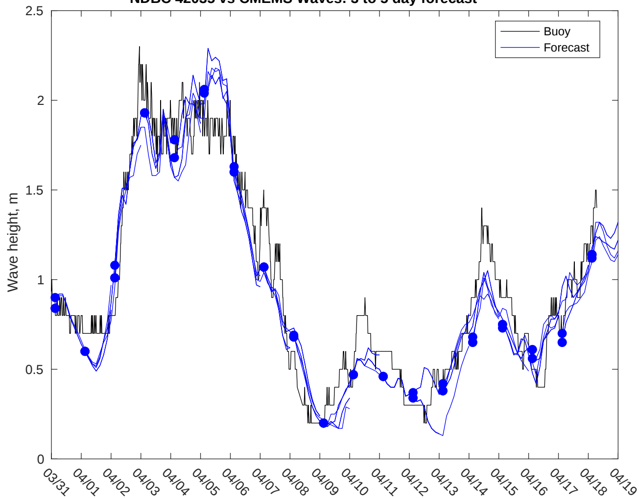
NDBC 42035 vs CMEMS Waves: 3 to 5 day forecast
