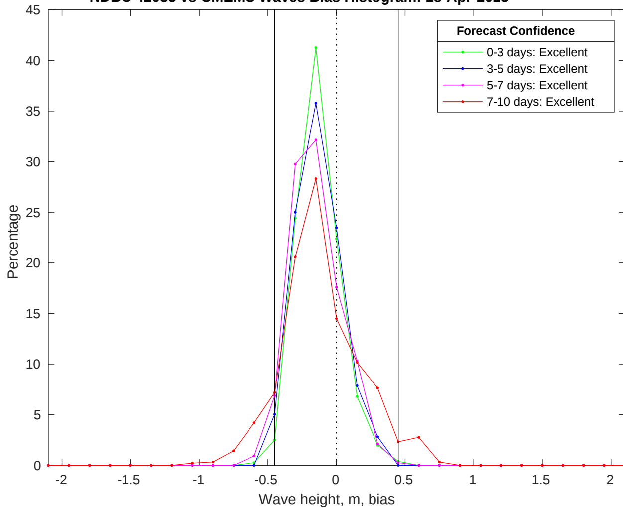
NDBC 42035 vs CMEMS Waves Bias Histogram: 18-Apr-2025
