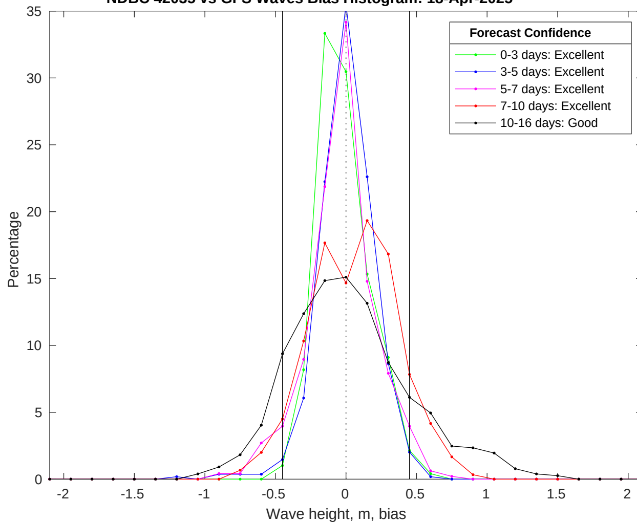
NDBC 42035 vs GFS Waves Bias Histogram: 18-Apr-2025
