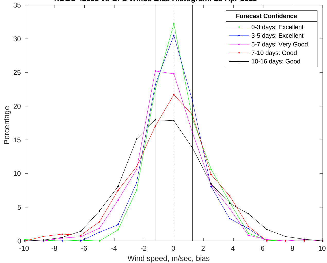
NDBC 42035 vs GFS Winds Bias Histogram: 18-Apr-2025
