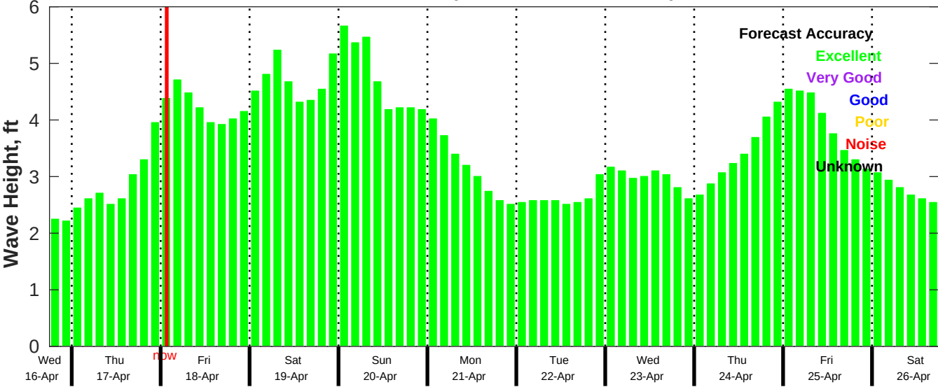
CMEMS Wave Forecast for NDBC 42035 from 16-Apr-2025 18:00:00 to 26-Apr-2025 18:00:00
