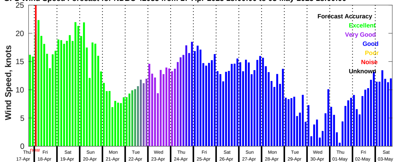
GFS Wind Speed Forecast for NDBC 42035 from 17-Apr-2025 18:00:00 to 03-May-2025 18:00:00
