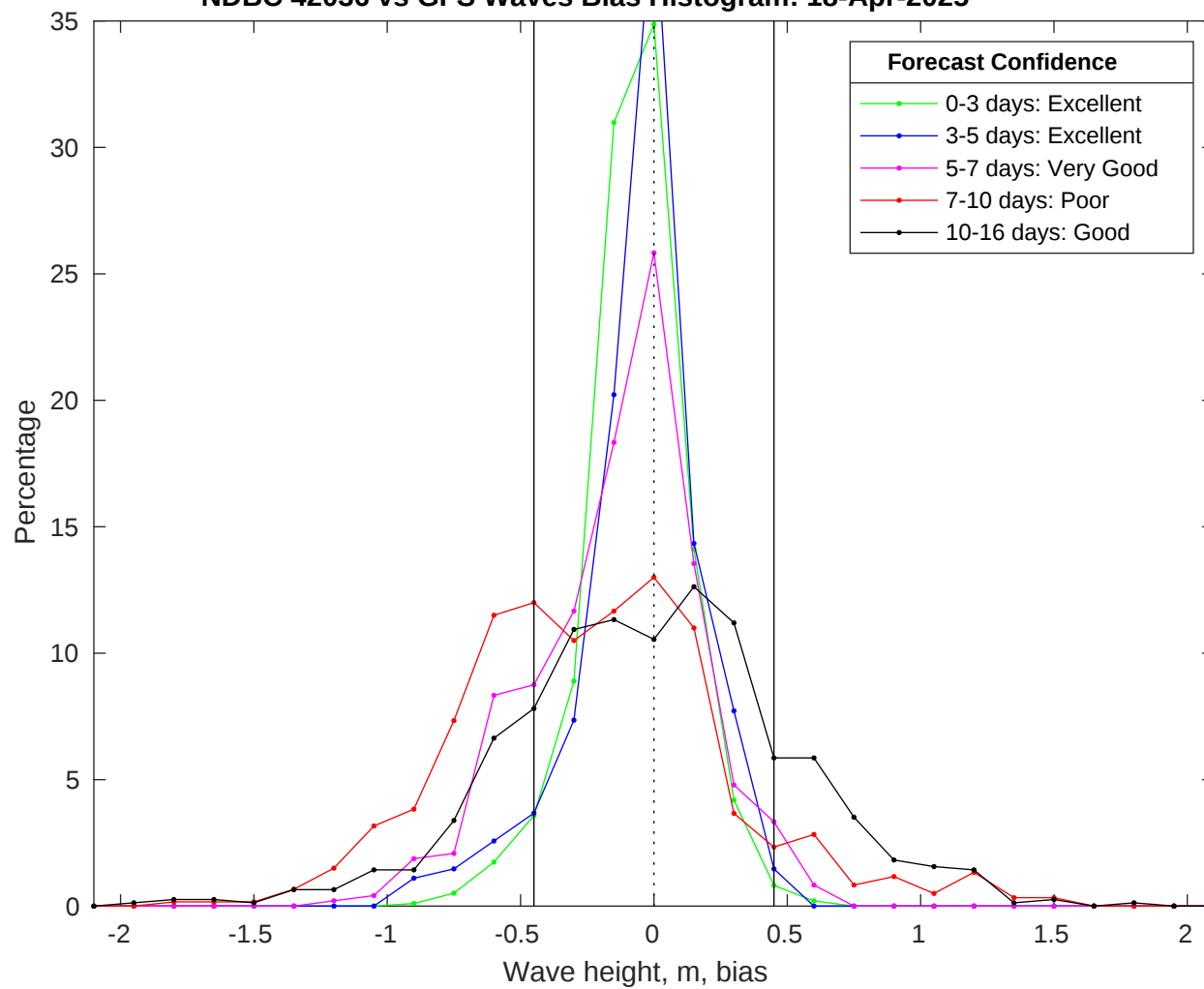
NDBC 42036 vs GFS Waves Bias Histogram: 18-Apr-2025
