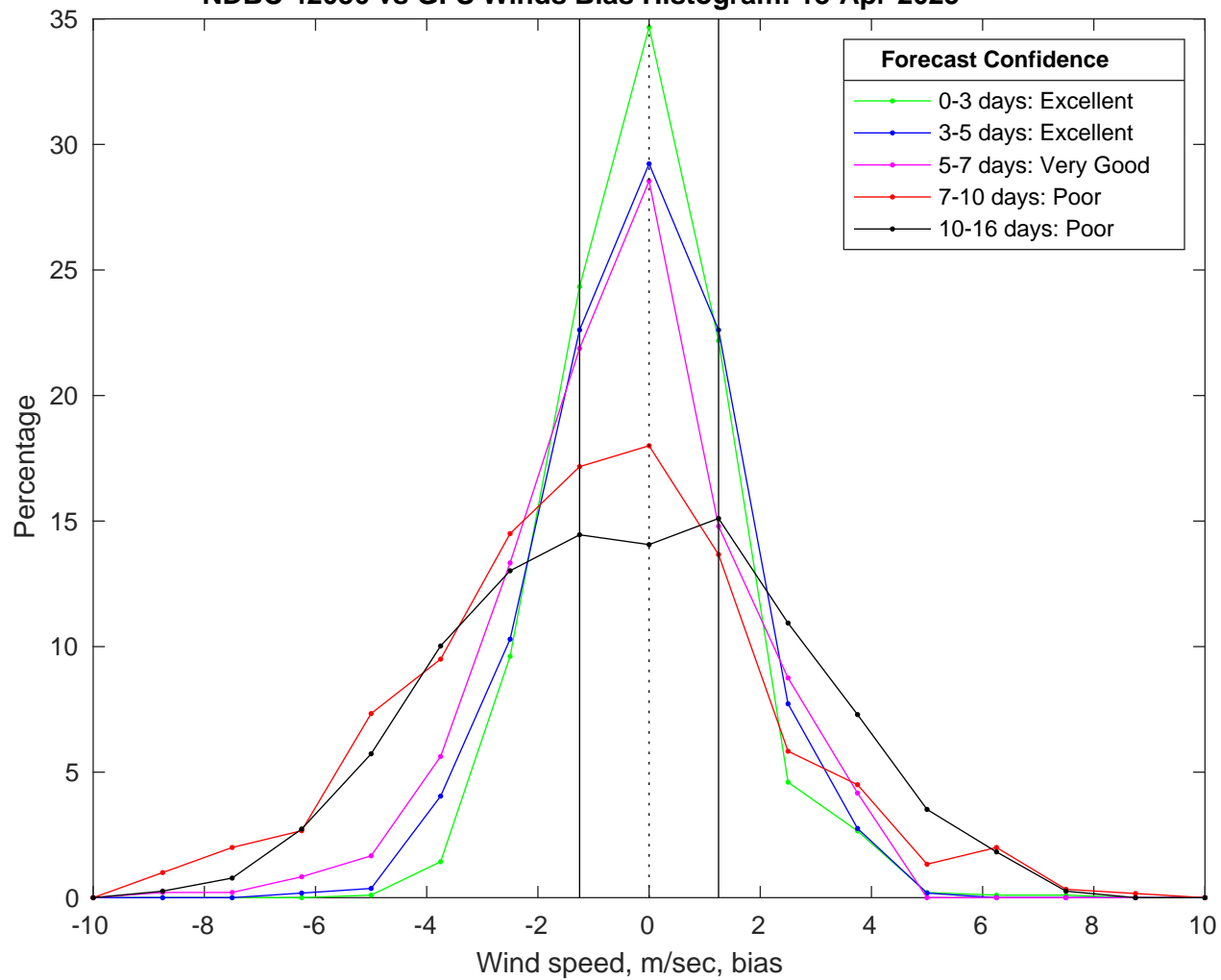
NDBC 42036 vs GFS Winds Bias Histogram: 18-Apr-2025
