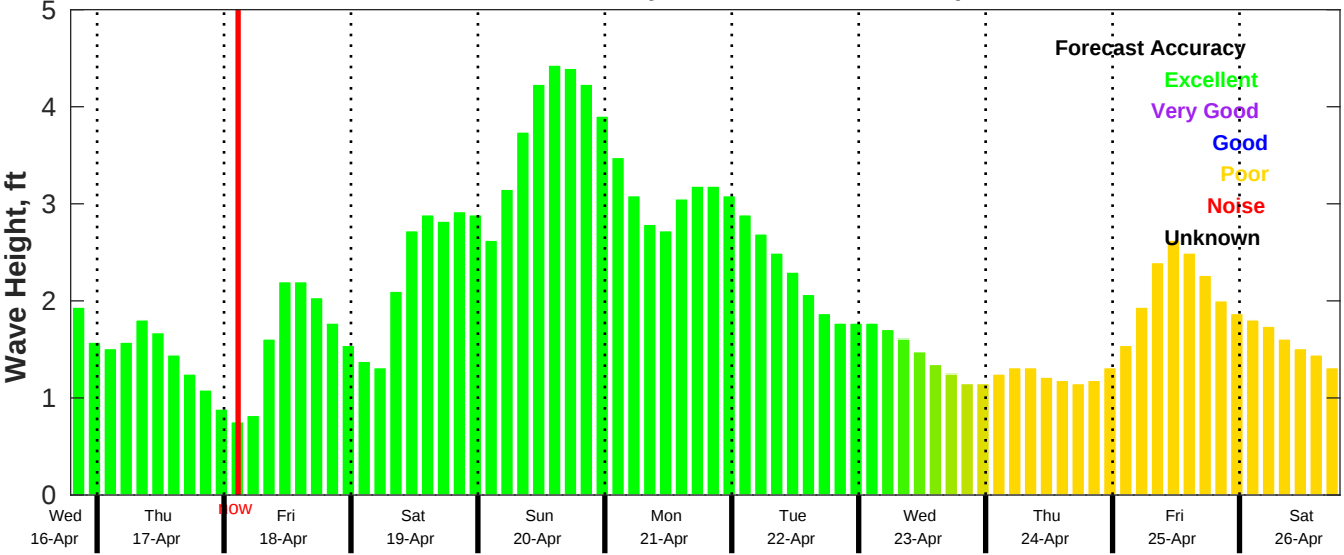
CMEMS Wave Forecast for NDBC 42036 from 16-Apr-2025 19:00:00 to 26-Apr-2025 19:00:00
