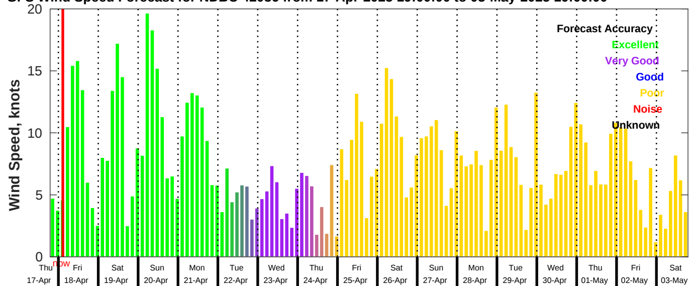
GFS Wind Speed Forecast for NDBC 42036 from 17-Apr-2025 19:00:00 to 03-May-2025 19:00:00
