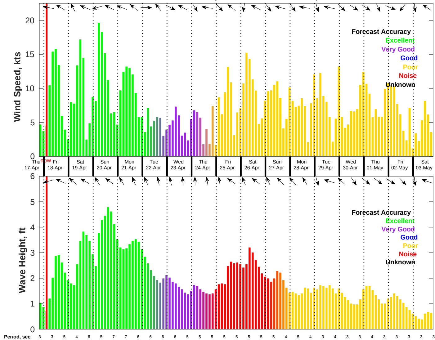
Wind & Wave Forecast for NDBC 42036 from 17-Apr-2025 19:00:00 to 03-May-2025 19:00:00
