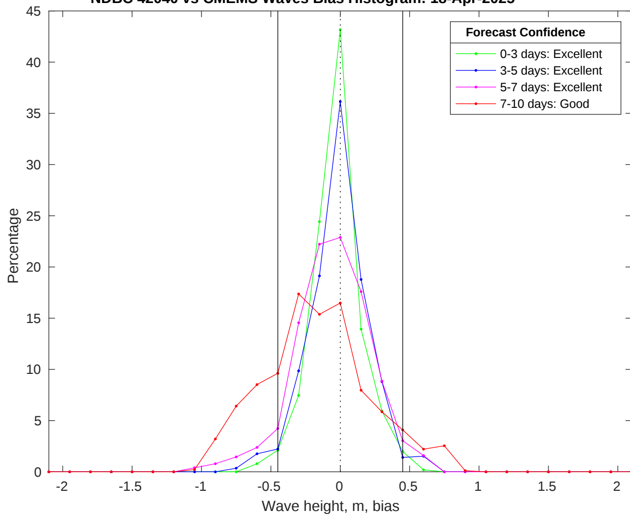
NDBC 42040 vs CMEMS Waves Bias Histogram: 18-Apr-2025
