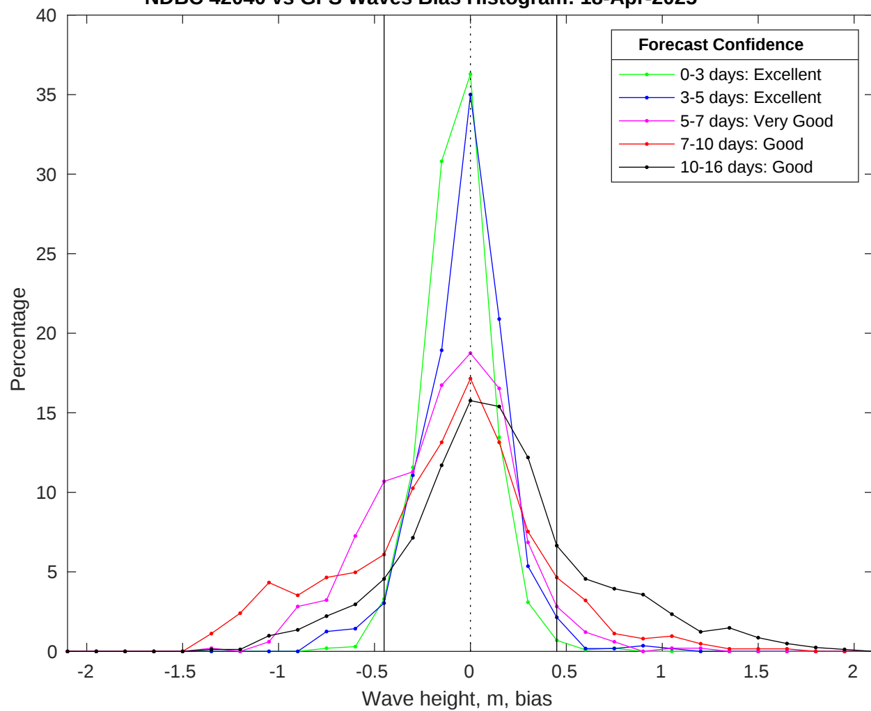
NDBC 42040 vs GFS Waves Bias Histogram: 18-Apr-2025
