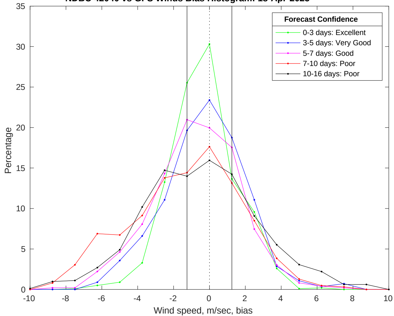
NDBC 42040 vs GFS Winds Bias Histogram: 18-Apr-2025
