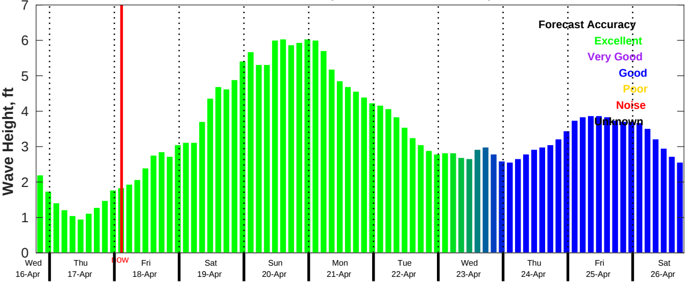
CMEMS Wave Forecast for NDBC 42040 from 16-Apr-2025 19:00:00 to 26-Apr-2025 19:00:00
