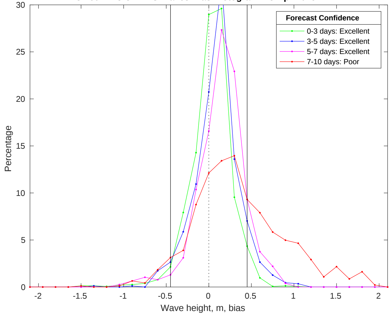
NDBC 46011 vs CMEMS Waves Bias Histogram: 18-Apr-2025
