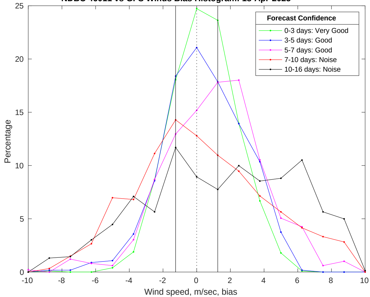
NDBC 46011 vs GFS Winds Bias Histogram: 18-Apr-2025
