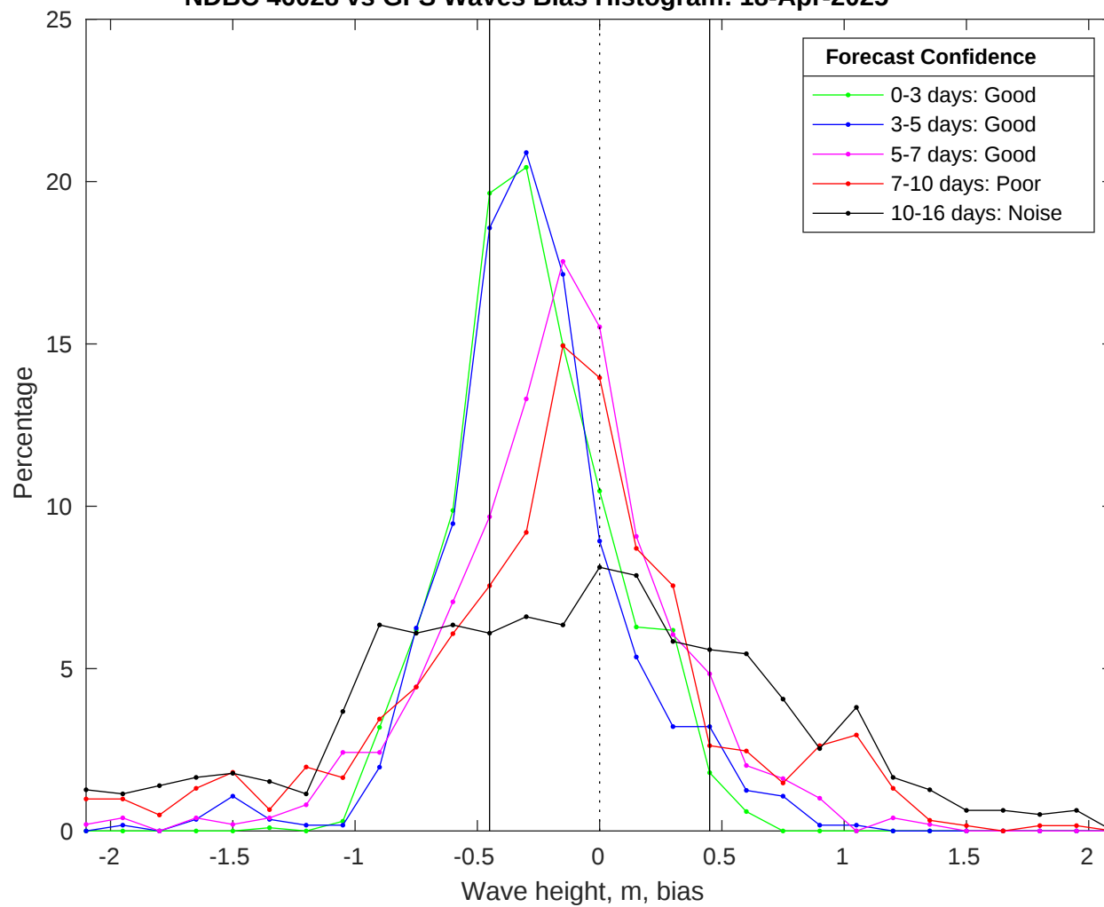
NDBC 46028 vs GFS Waves Bias Histogram: 18-Apr-2025
