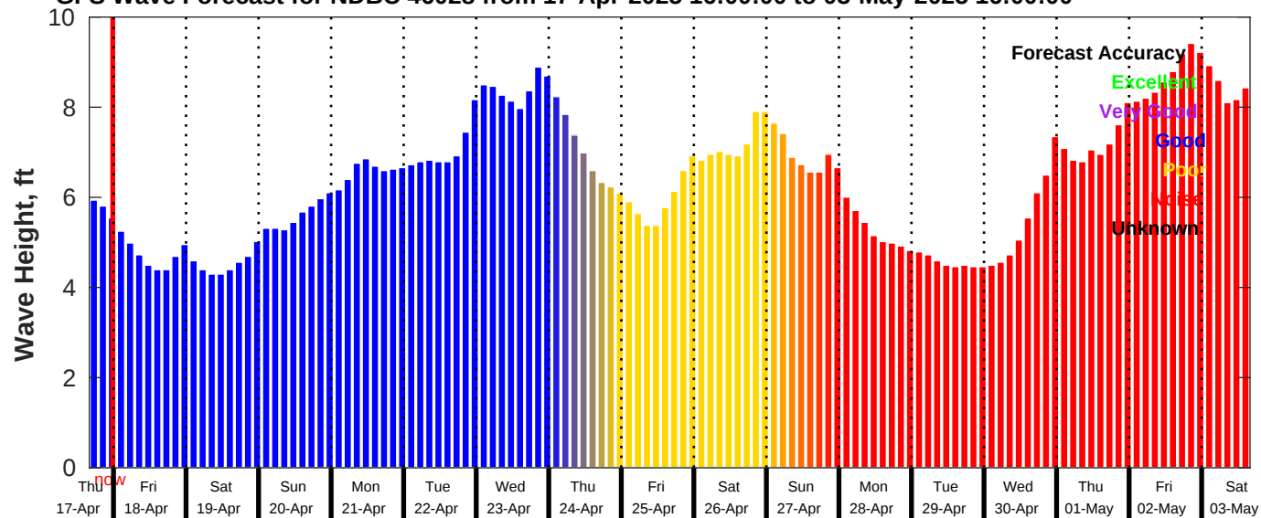
GFS Wave Forecast for NDBC 46028 from 17-Apr-2025 16:00:00 to 03-May-2025 16:00:00
