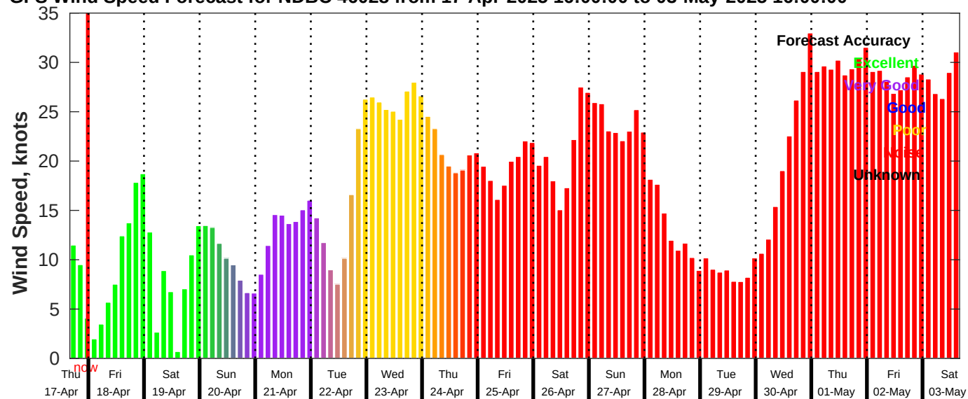
GFS Wind Speed Forecast for NDBC 46028 from 17-Apr-2025 16:00:00 to 03-May-2025 16:00:00
