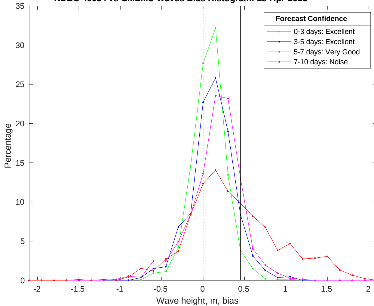
NDBC 46054 vs CMEMS Waves Bias Histogram: 18-Apr-2025
