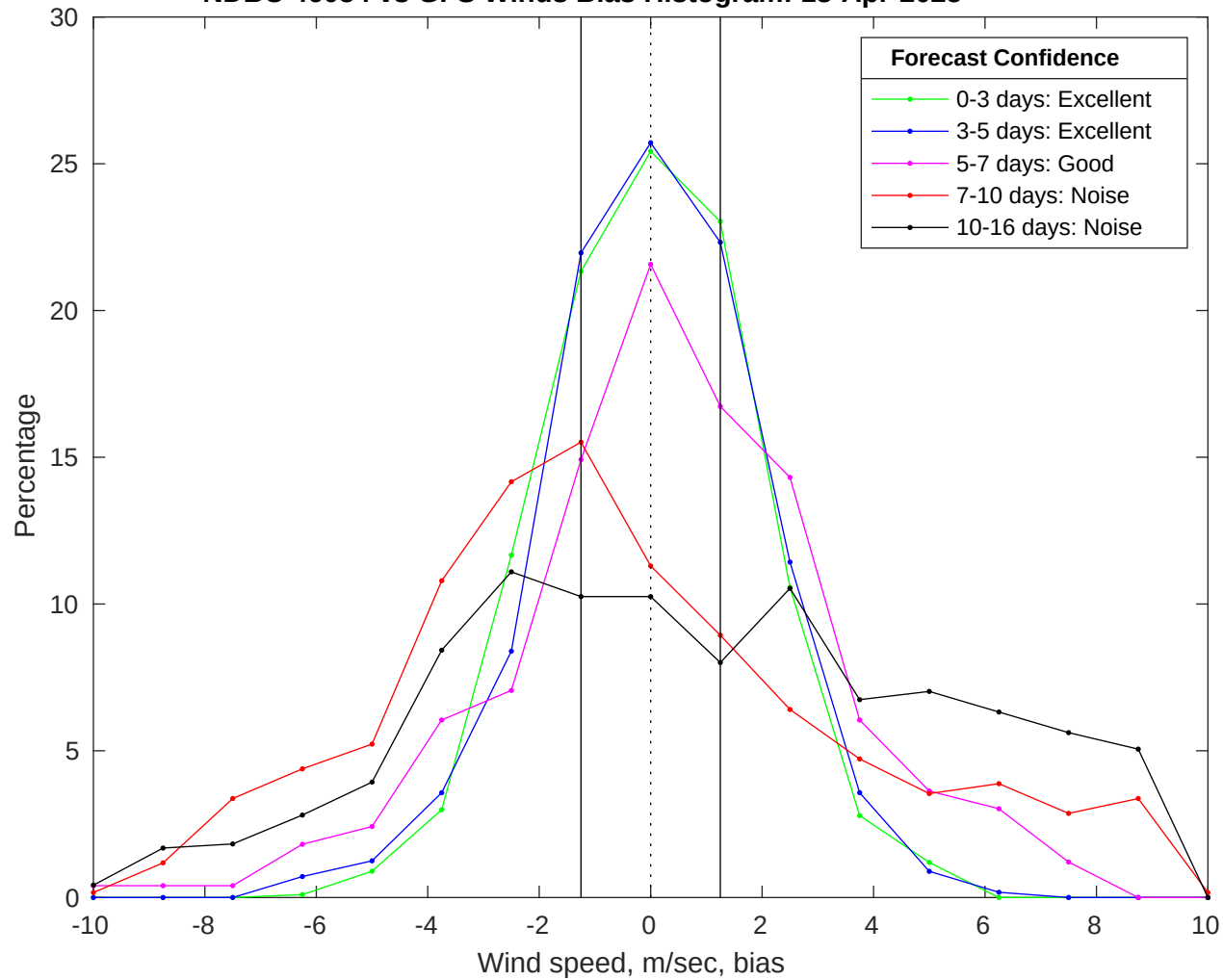
NDBC 46054 vs GFS Winds Bias Histogram: 18-Apr-2025
