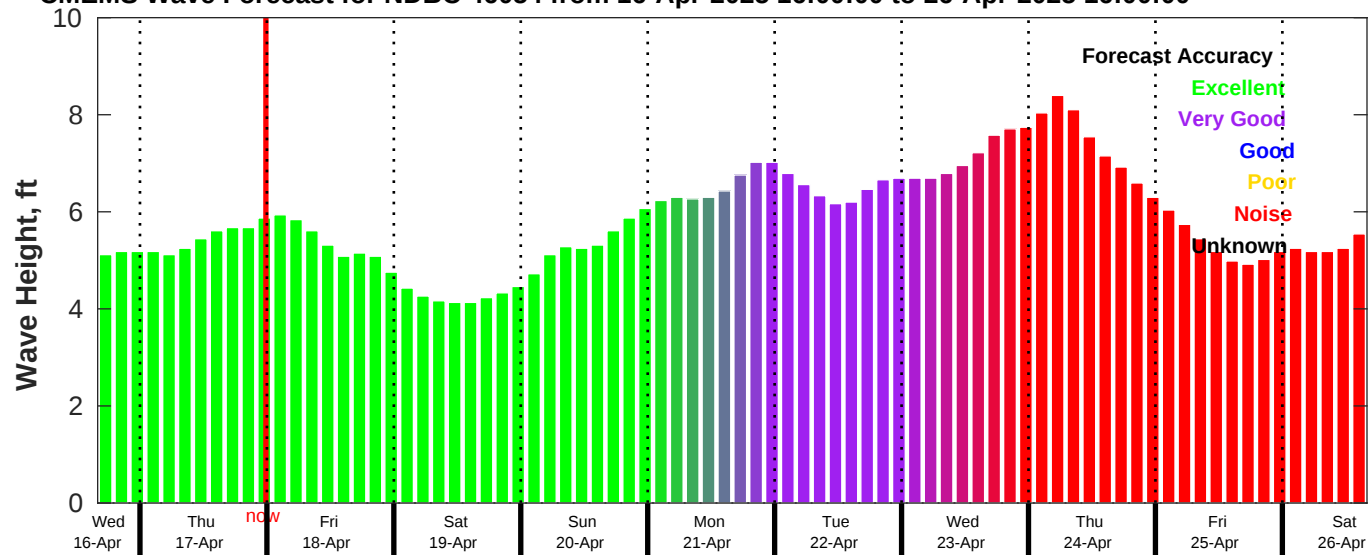
CMEMS Wave Forecast for NDBC 46054 from 16-Apr-2025 16:00:00 to 26-Apr-2025 16:00:00
