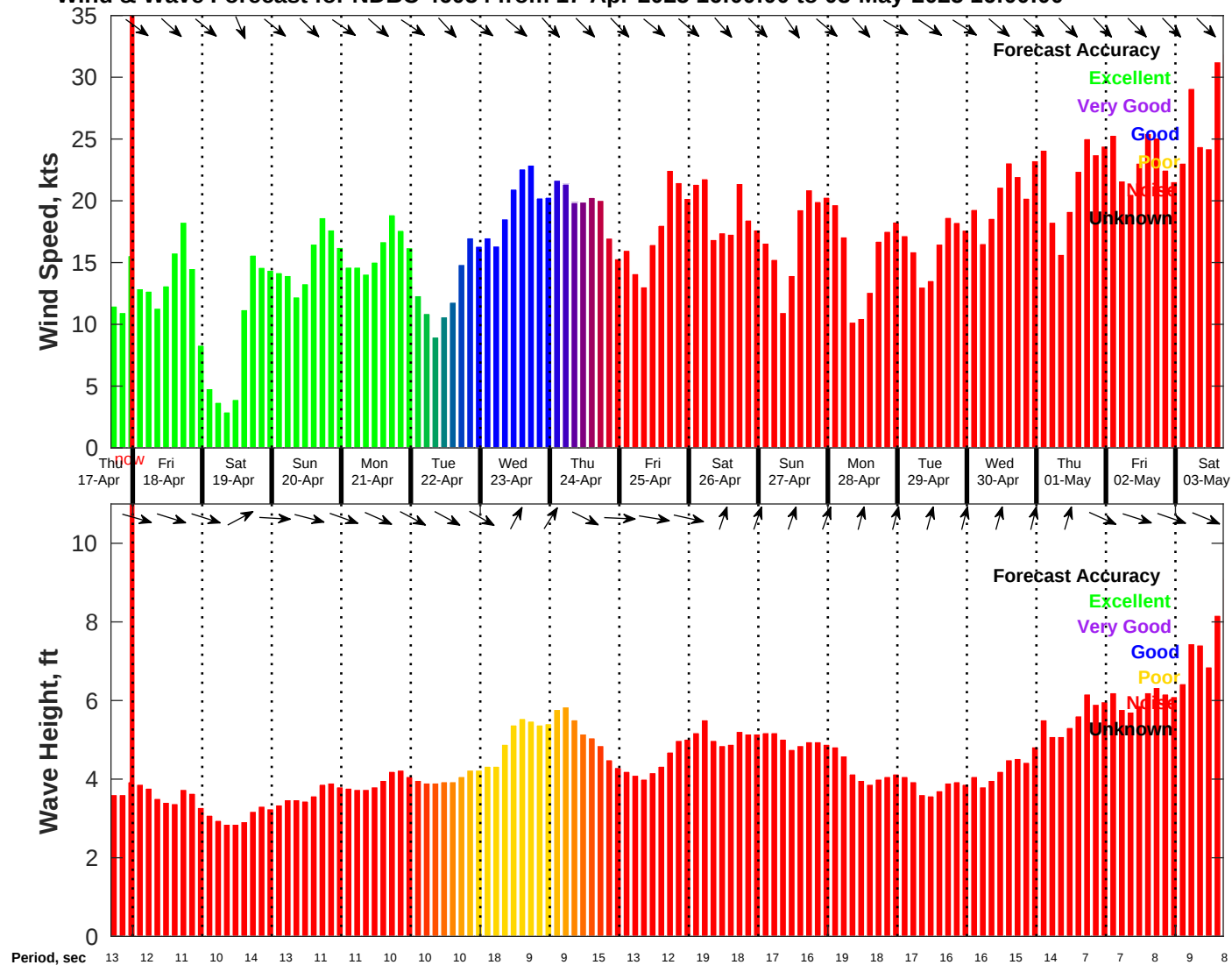
Wind & Wave Forecast for NDBC 46054 from 17-Apr-2025 16:00:00 to 03-May-2025 16:00:00
