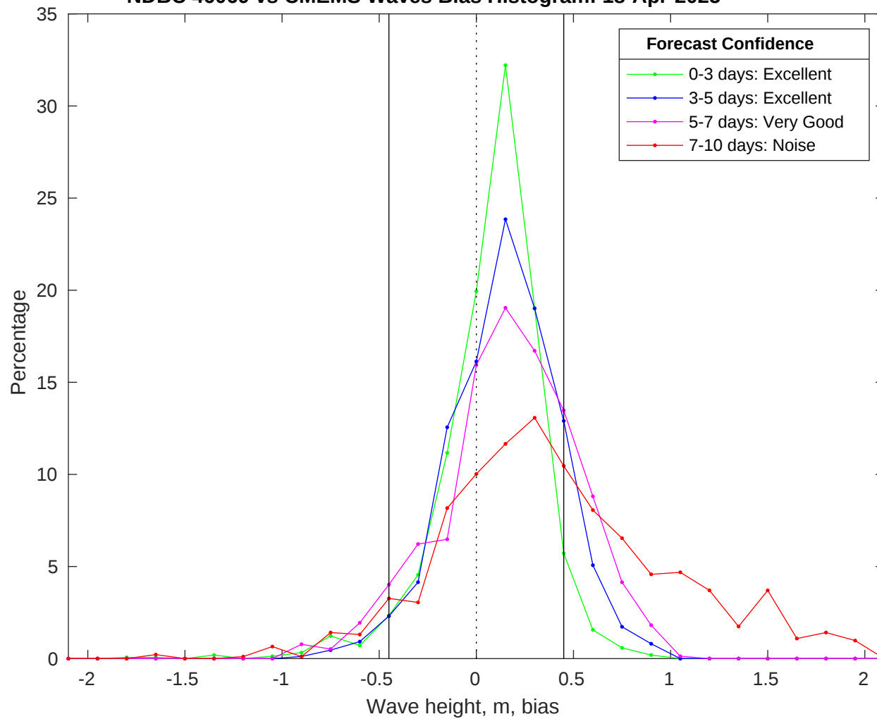
NDBC 46069 vs CMEMS Waves Bias Histogram: 18-Apr-2025
