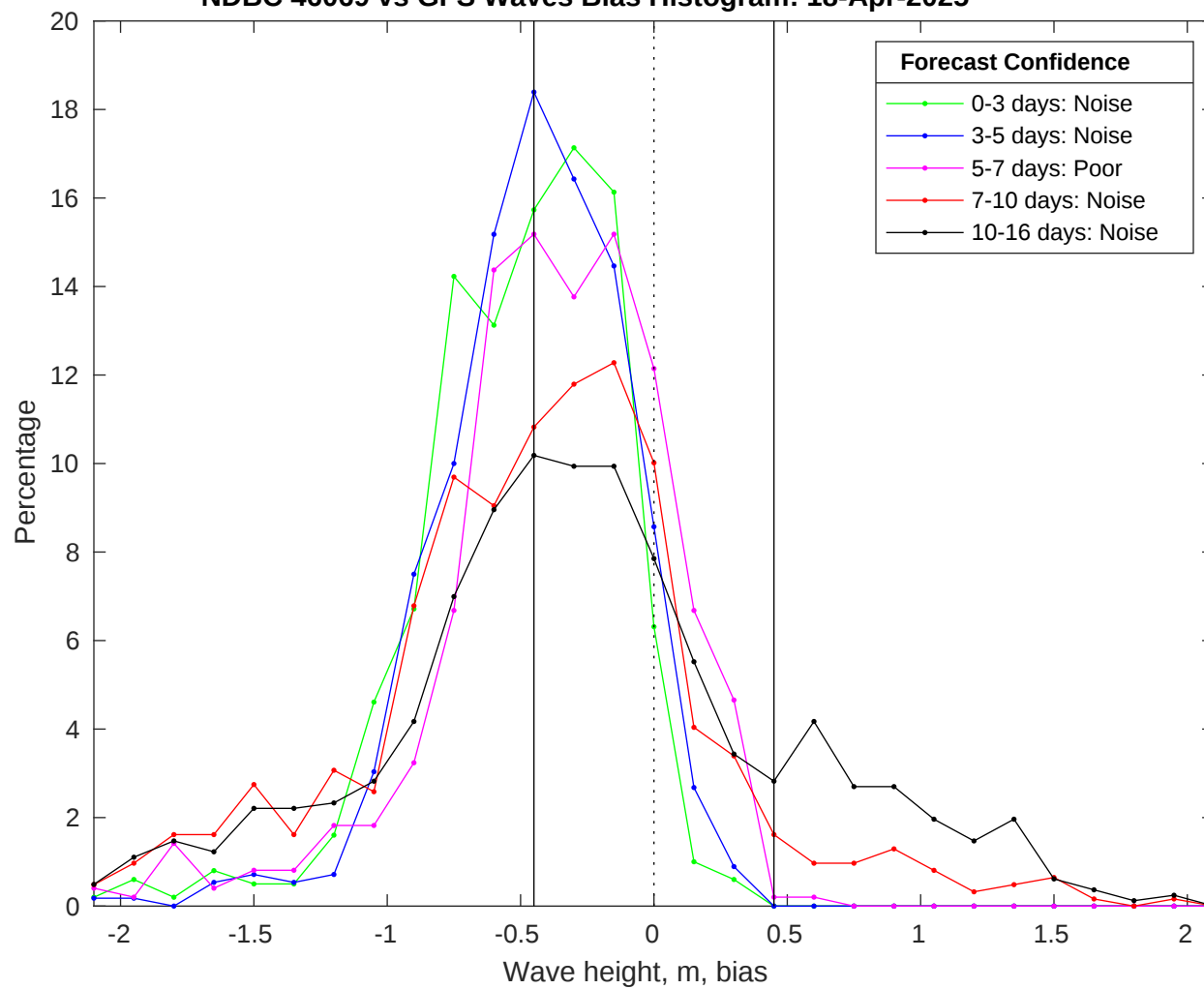
NDBC 46069 vs GFS Waves Bias Histogram: 18-Apr-2025
