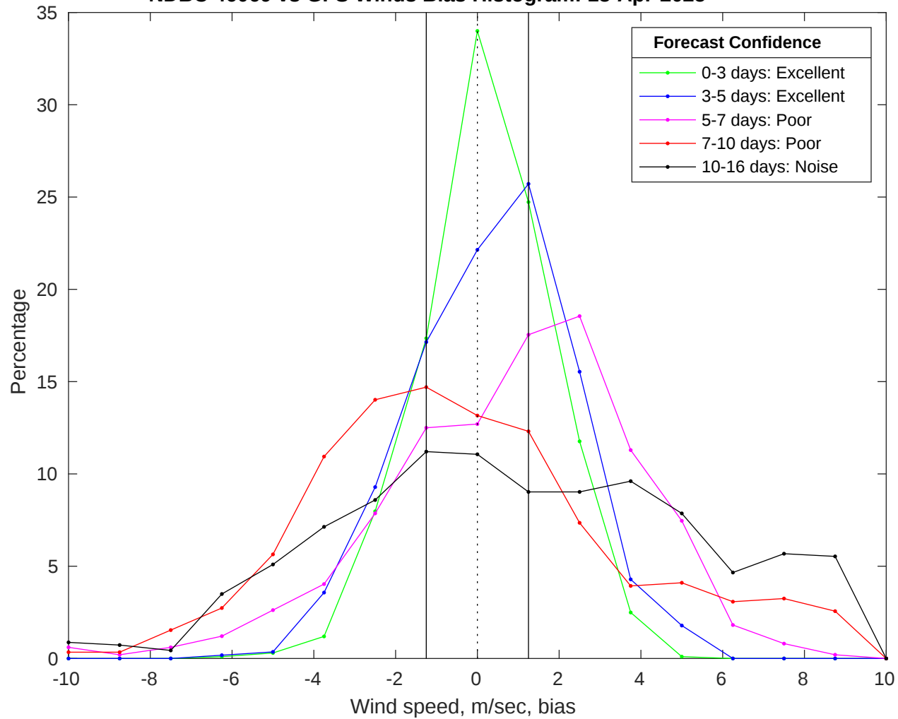
NDBC 46069 vs GFS Winds Bias Histogram: 18-Apr-2025
