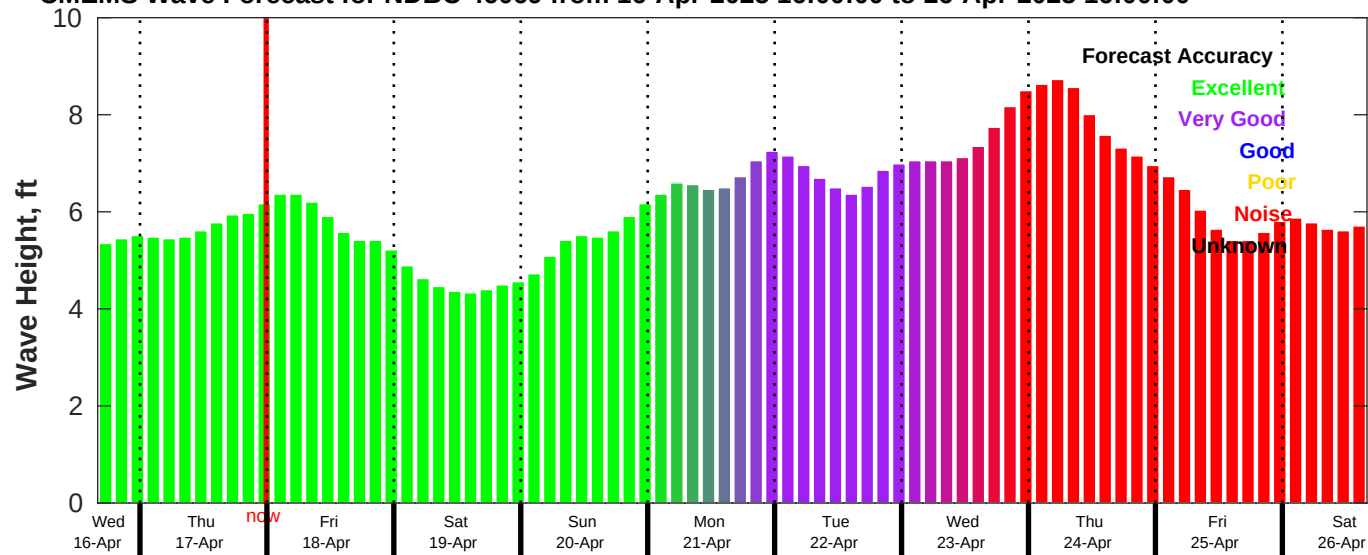
CMEMS Wave Forecast for NDBC 46069 from 16-Apr-2025 16:00:00 to 26-Apr-2025 16:00:00
