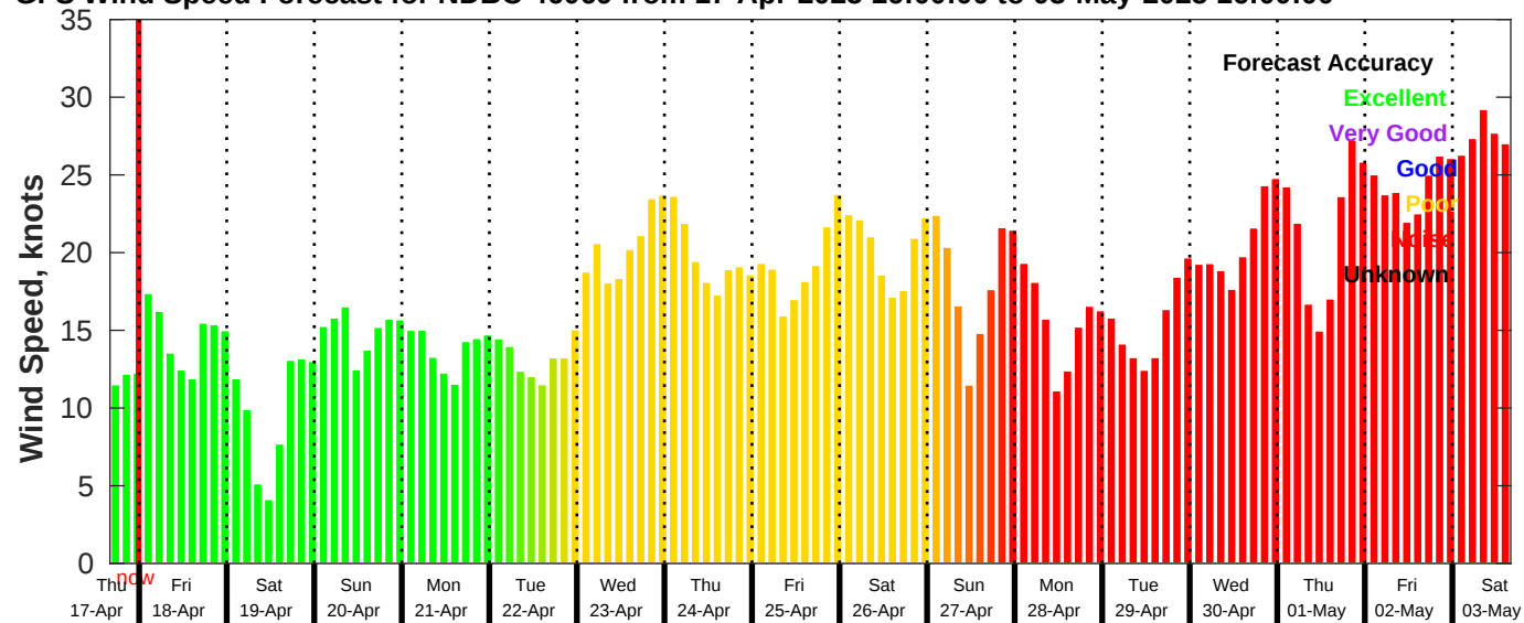
GFS Wind Speed Forecast for NDBC 46069 from 17-Apr-2025 16:00:00 to 03-May-2025 16:00:00
