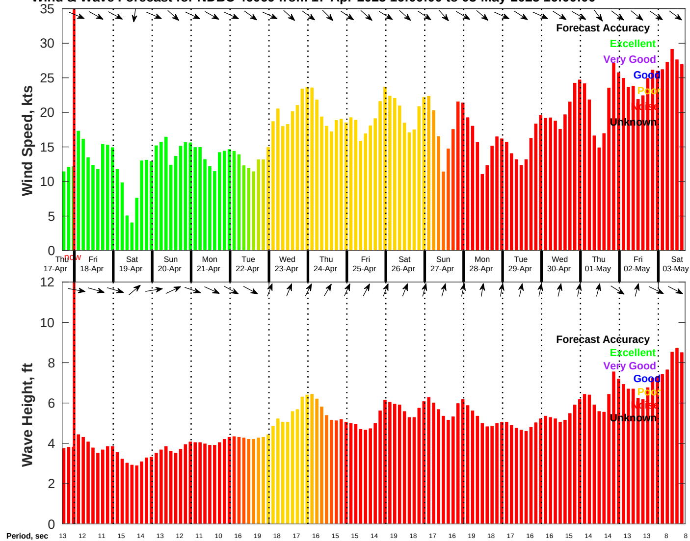
Wind & Wave Forecast for NDBC 46069 from 17-Apr-2025 16:00:00 to 03-May-2025 16:00:00
