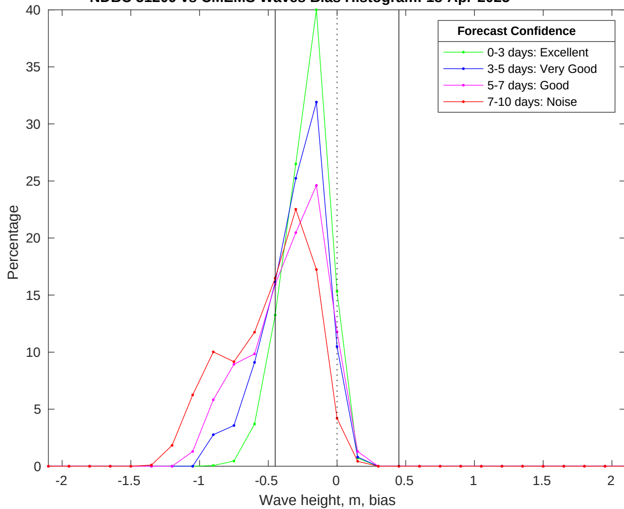
NDBC 51209 vs CMEMS Waves Bias Histogram: 18-Apr-2025
