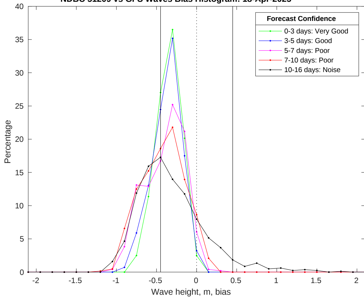
NDBC 51209 vs GFS Waves Bias Histogram: 18-Apr-2025
