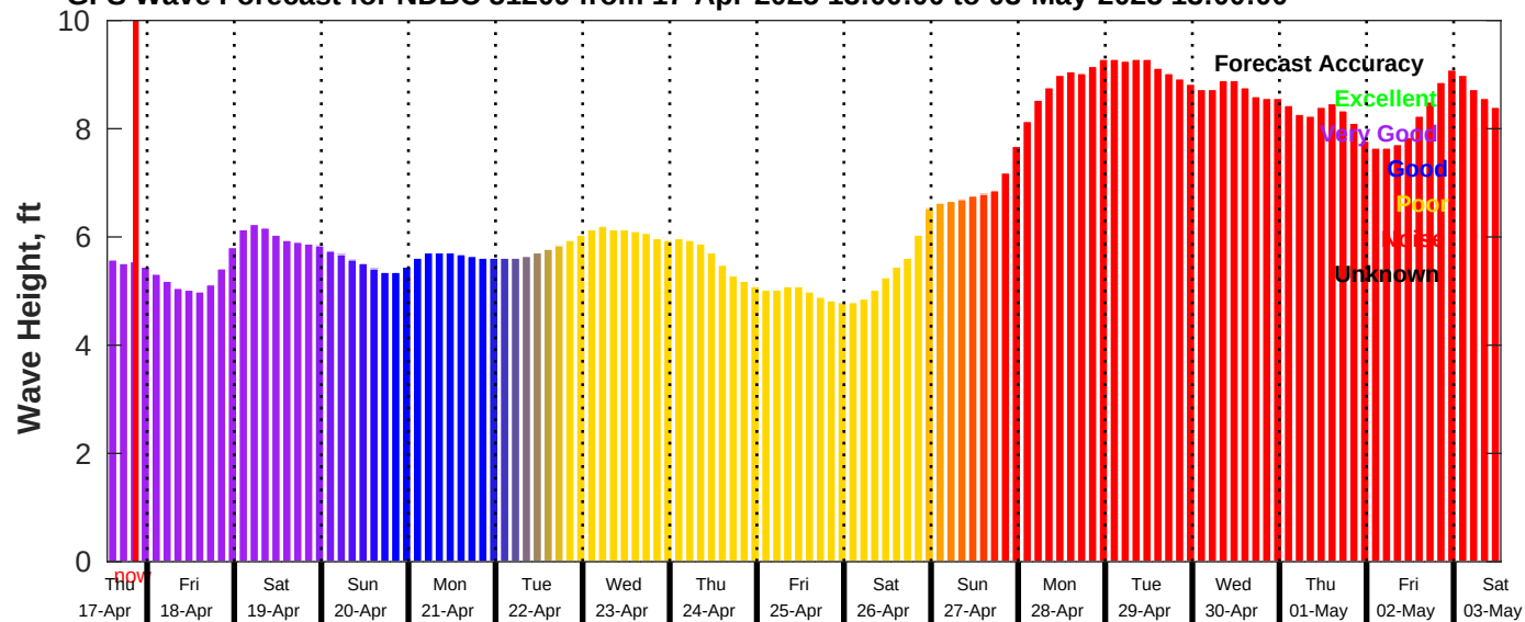
GFS Wave Forecast for NDBC 51209 from 17-Apr-2025 13:00:00 to 03-May-2025 13:00:00
