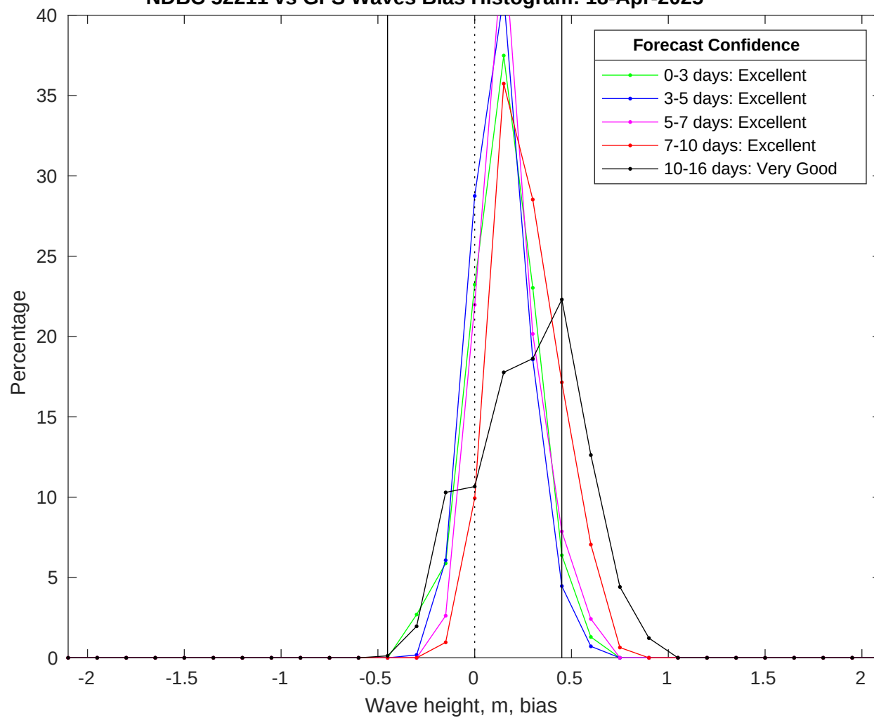
NDBC 52211 vs GFS Waves Bias Histogram: 18-Apr-2025
