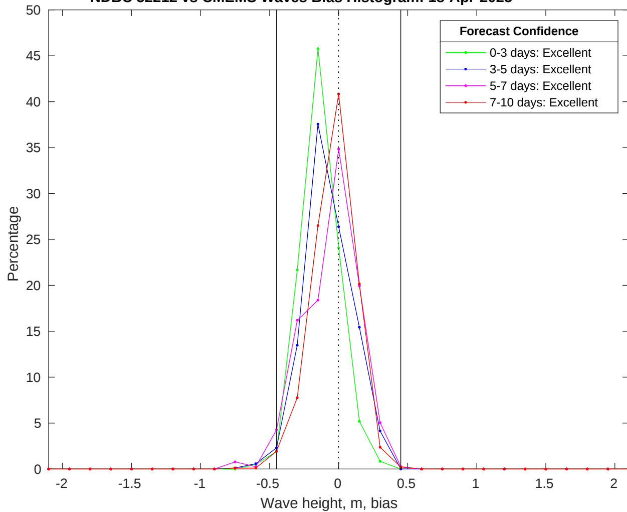
NDBC 52212 vs CMEMS Waves Bias Histogram: 18-Apr-2025
